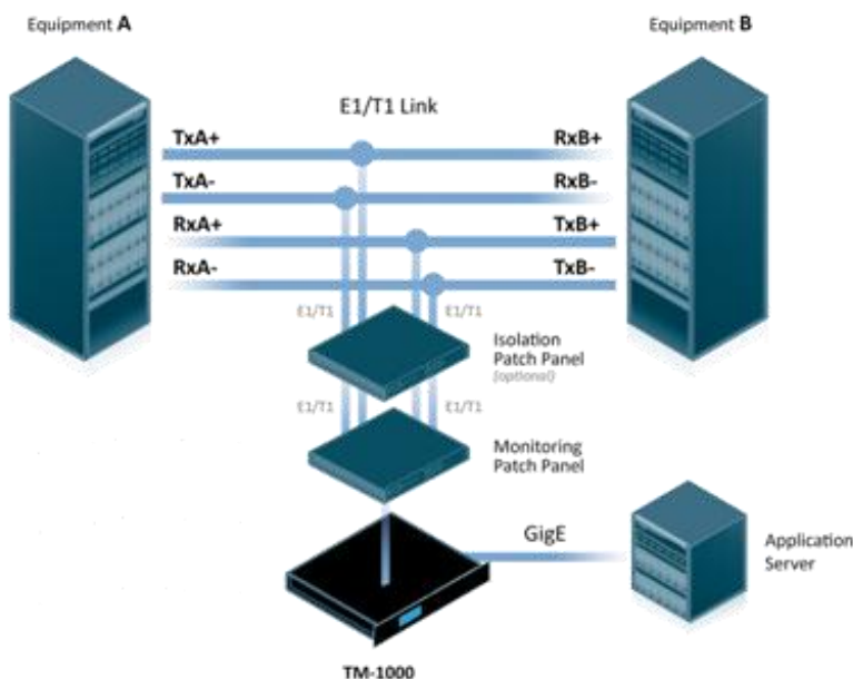
> Figure: sample integration of the Tmonitor TM1000
